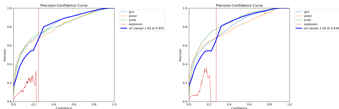
Figure 4.1: YOLO11s Precision Curve Figure 4.2: YOLOv8s Precision Curve
